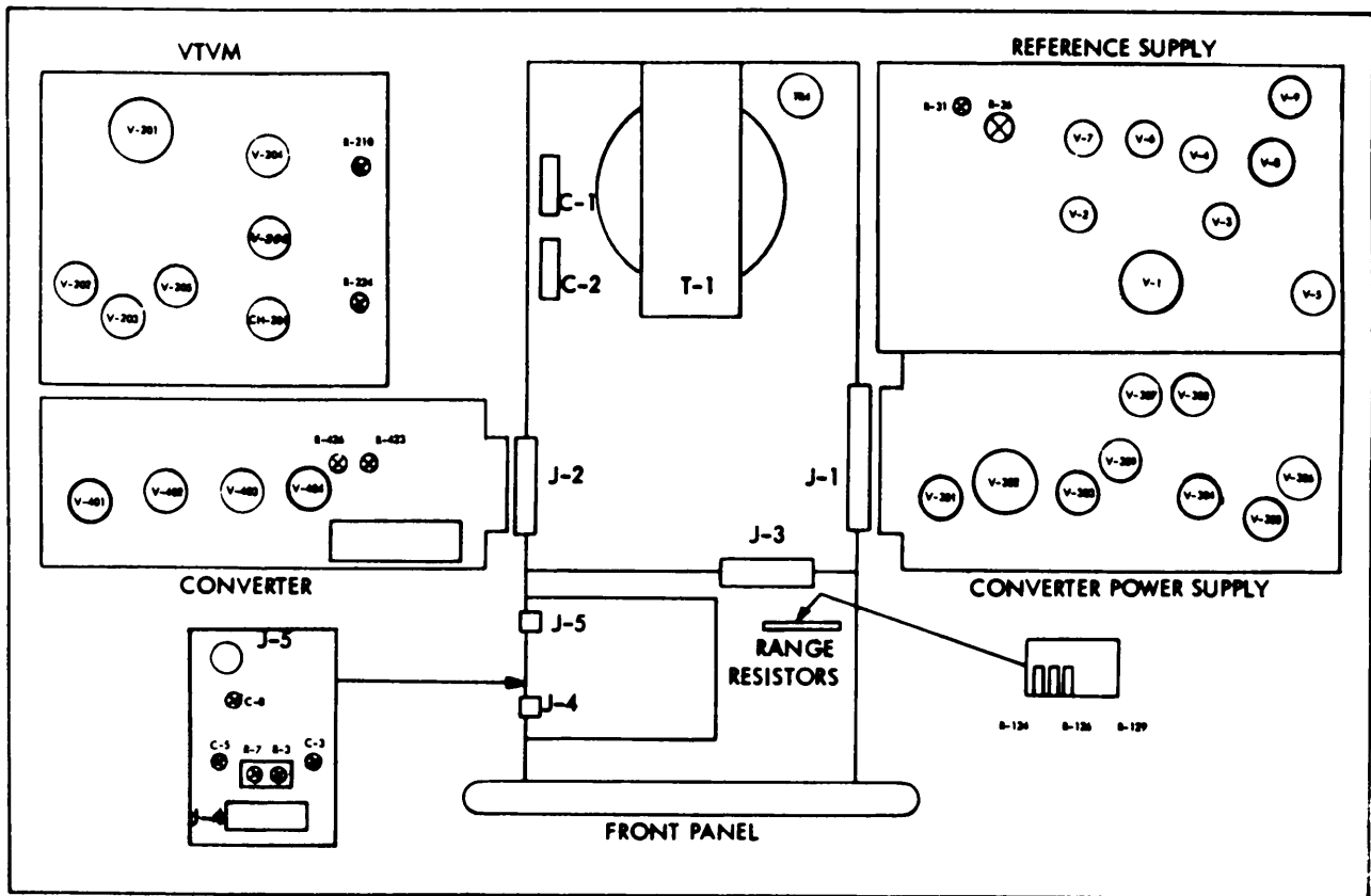
Figure 4-1. COMPONENT LOCATION
